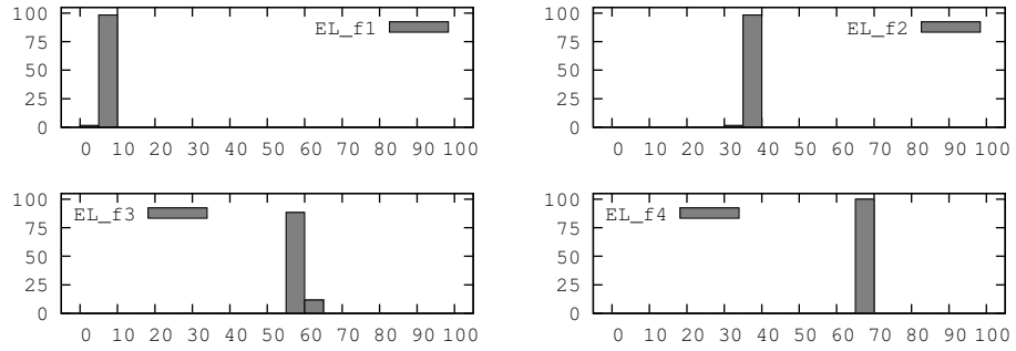
Figure 8: MAD-SADD performances in the high density scenario. The y axis represents percentages of (the total number of) nodes; in the x axis we have energy left percentage ( EL ).
