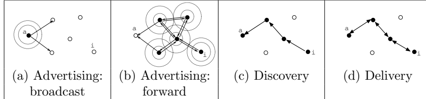
Figure 1: An example of MAD-SADD execution
