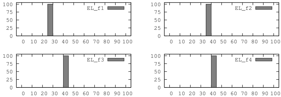
Figure 6: MAD-SADD performances in the low density scenario. The y axis represents percentages of (the total number of) nodes; in the x axis we have energy left percentage ( EL ).
