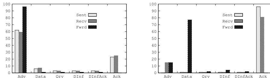
Figure 5: MAD-SADD performances on packets with (left) and without (right) Bloom filter. The y axis shows percentages of (the total number of) nodes.
