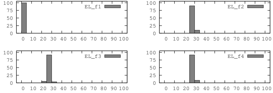
Figure 7: MAD-SADD performances in the medium density scenario. The y axis represents percentages of (the total number of) nodes; in the x axis we have energy left percentage ( EL ).
