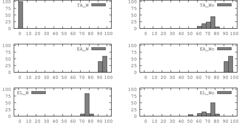
Figure 4: Bloom filter performances on advertising and energy. The y axis represents percentages of (the total number of) nodes. The x axis represents: total advertising percentage , effective advertising percentage , energy left percentage respectively in the first, second, and third row.
